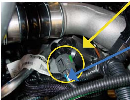
04.5 - 05 EGR Solenoid Module (passenger side)
